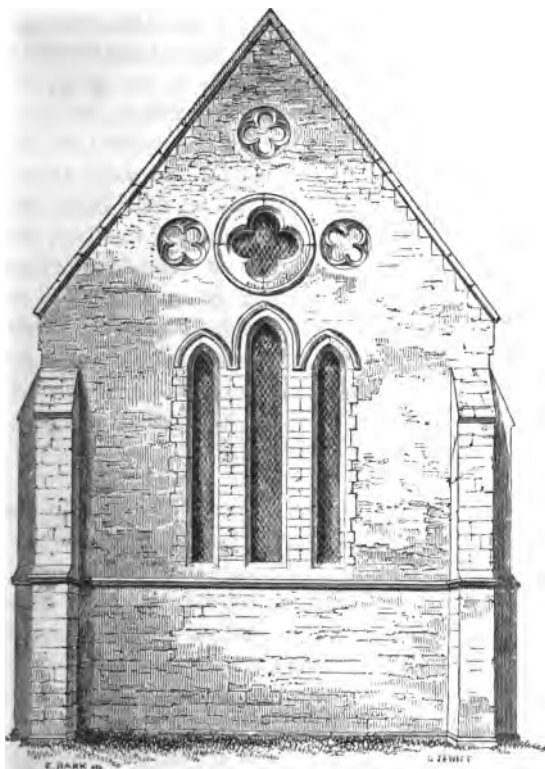
118. Strixton, Northamptonshire, c. 1220.
